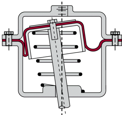
Cocked Piston
